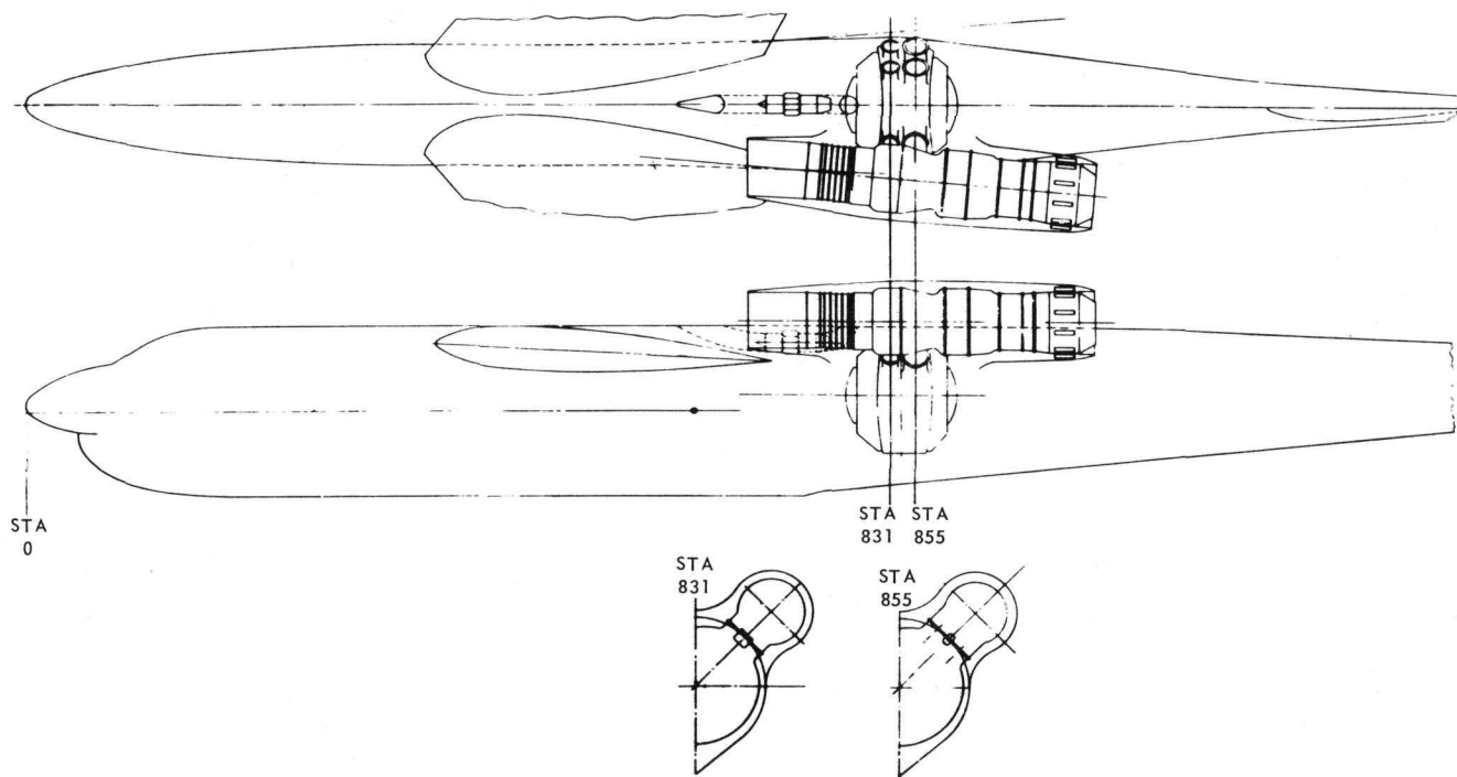
Fig. 2.11 - Modified AC-110 power-plant installation
