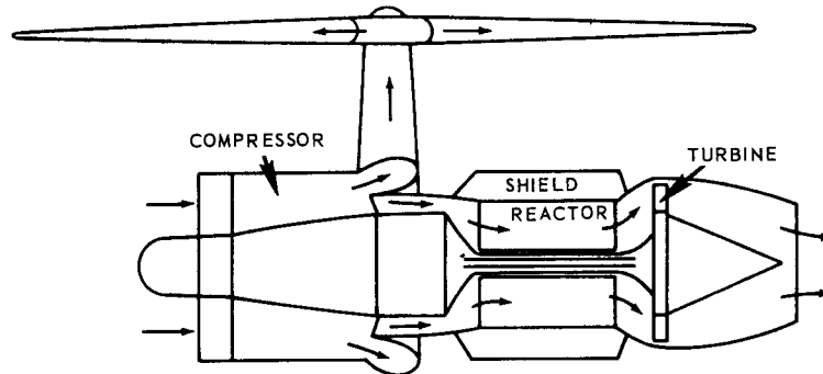
Fig. 6.2—Cold-cycle nuclear helicopter system
