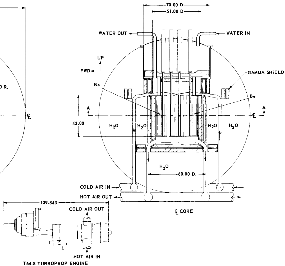
Fig. 10.1—Propulsion system proposal layout (629E288)
