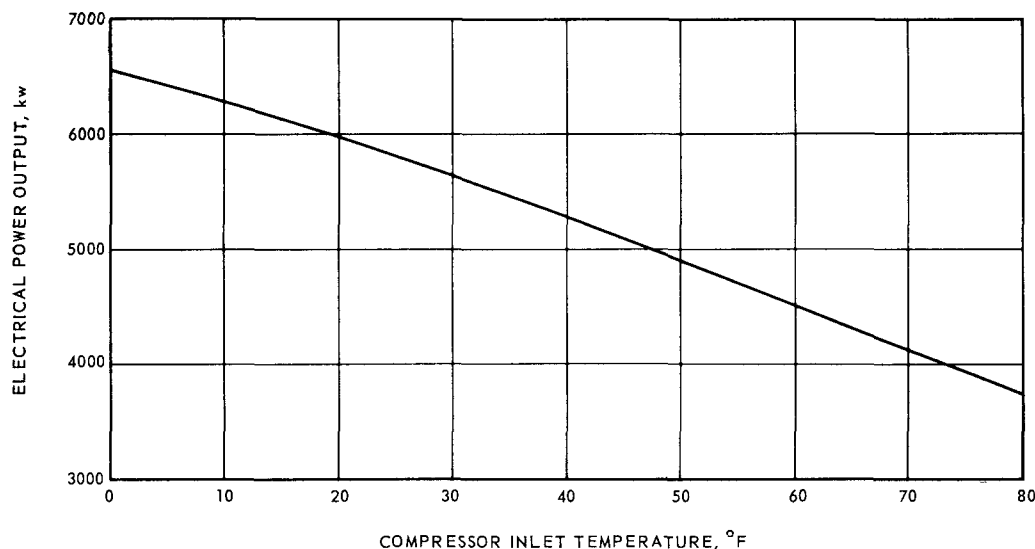
Fig. 8.3—Portable-power-plant power as a function of ambient temperature
