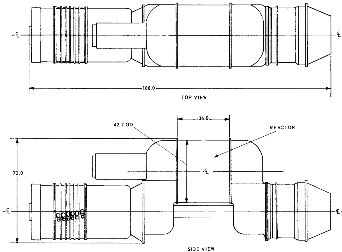
Fig. 4.10 -- Offset ceramic reactor with modified J79X207 engine
