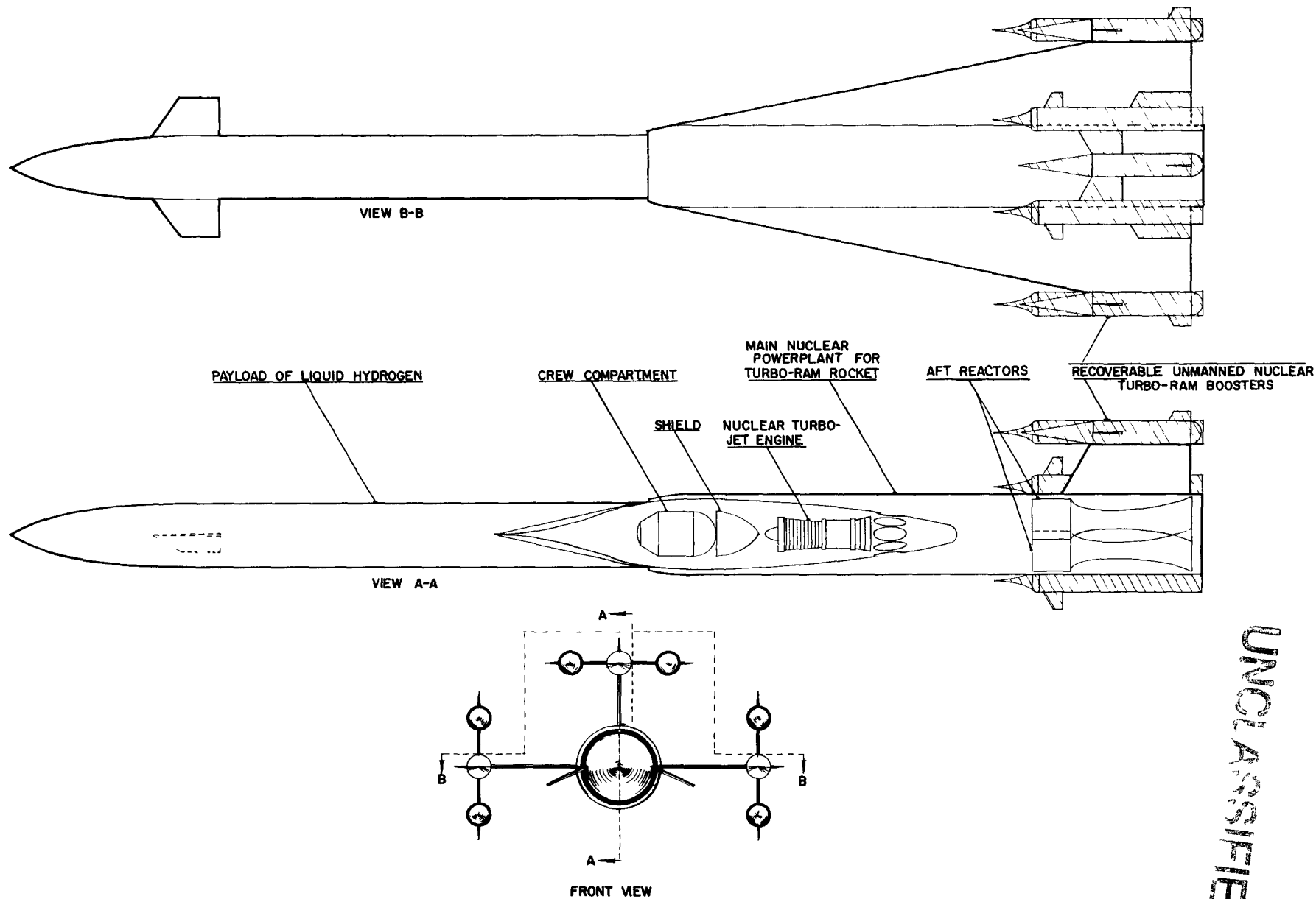
Fig. 12.1 - Nuclear-powered turbo-ram-rocket
