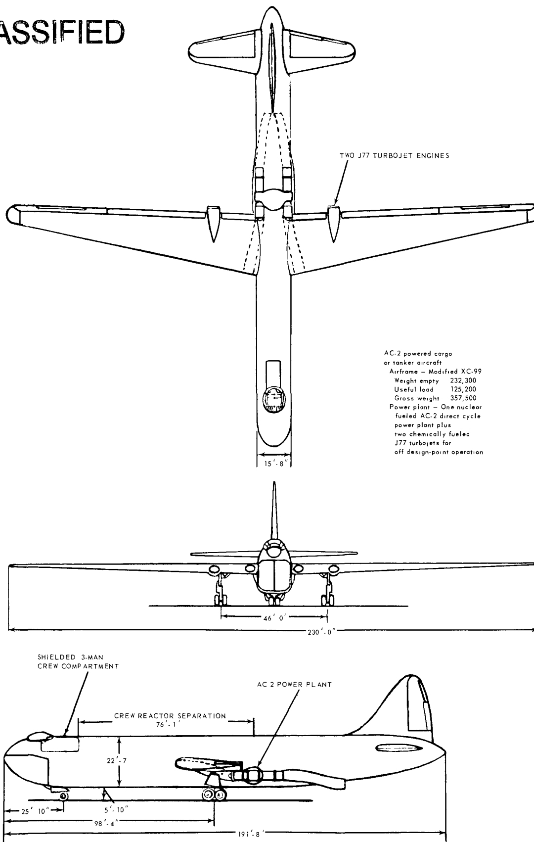
Fig. 2.1 - C-99 airplane - nuclear version
