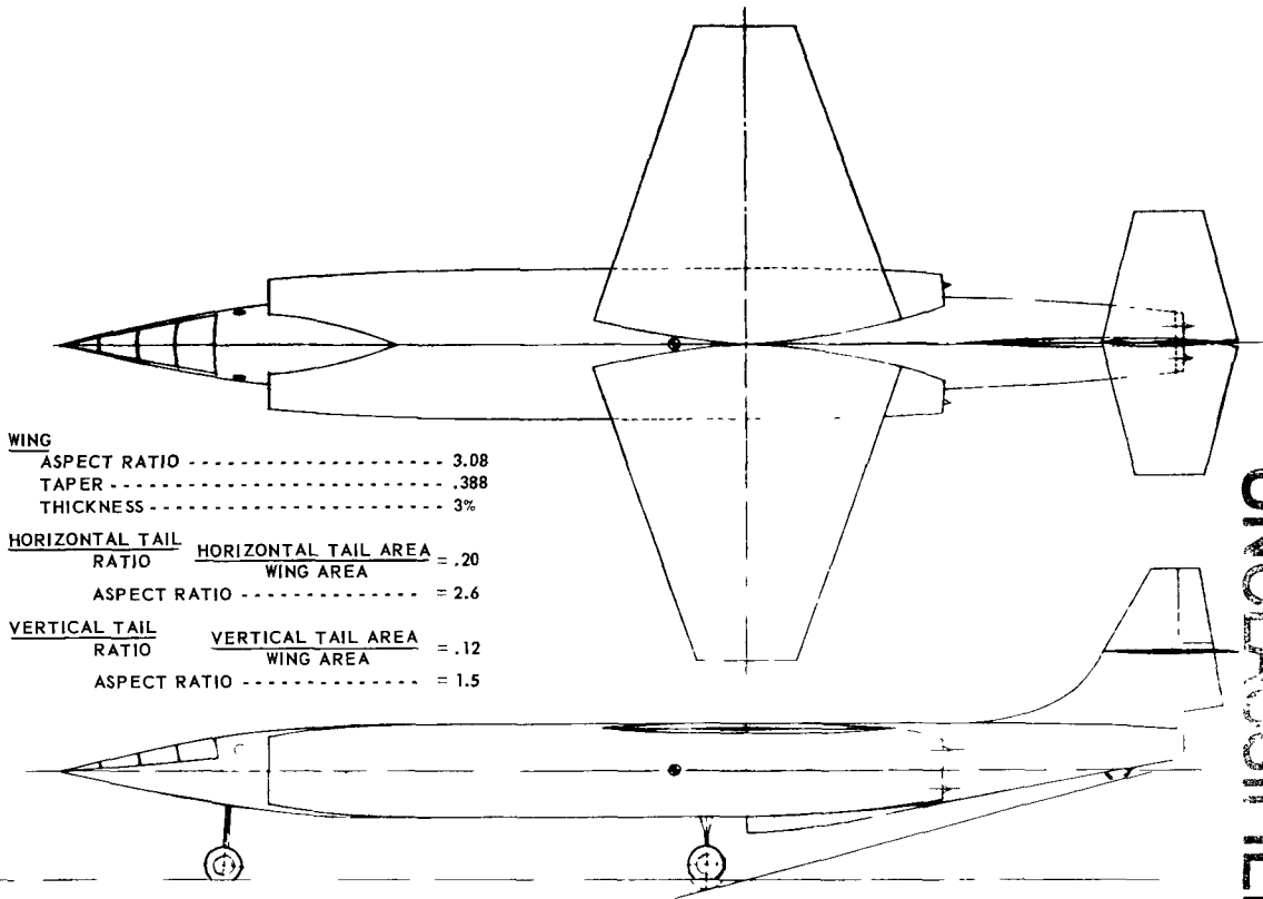
Fig. 3.1 - Supersonic nuclear-powered aircraft
