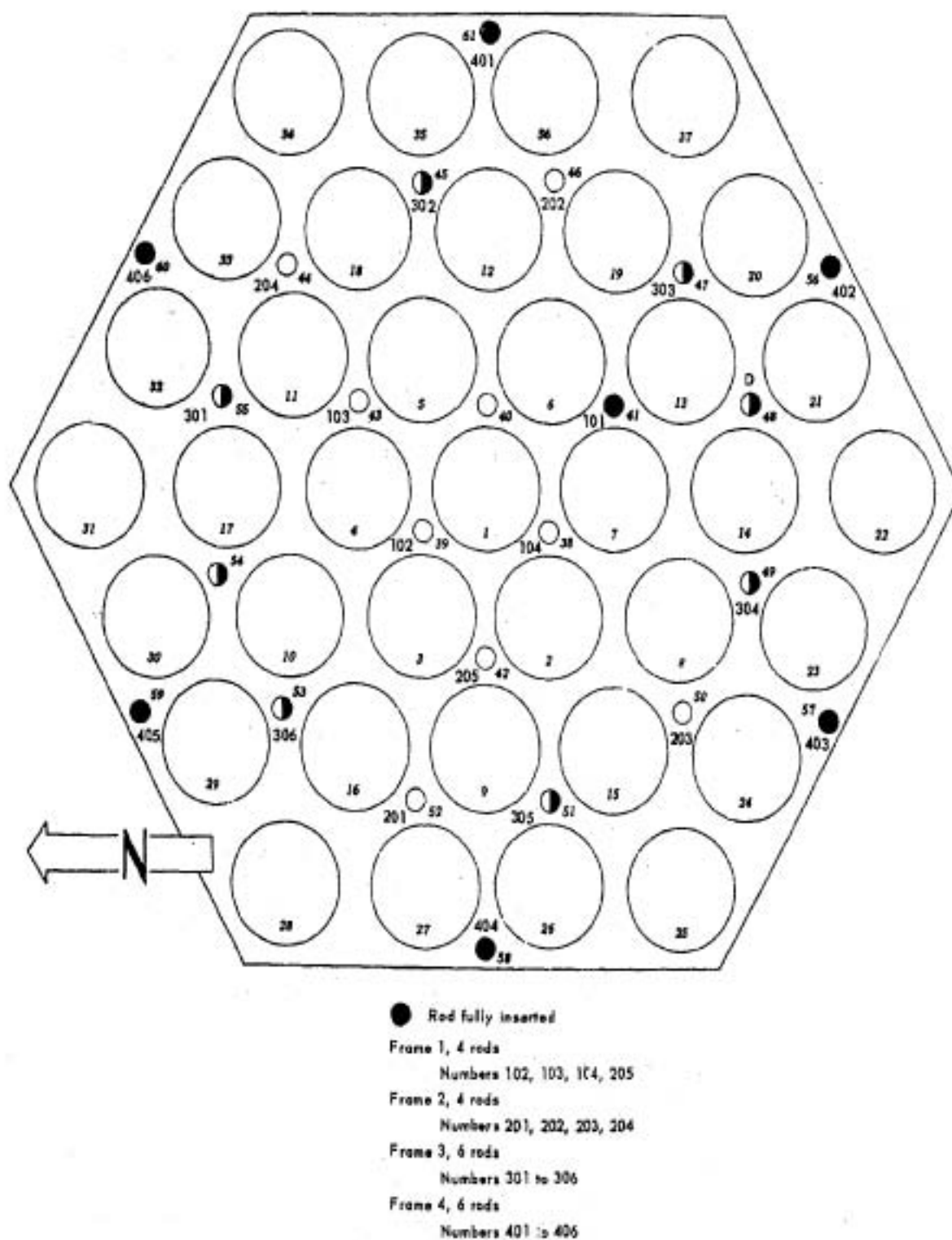
Figure 2-14 Rod Pattern for Series-28 Runs, Initial Engine Test #3
