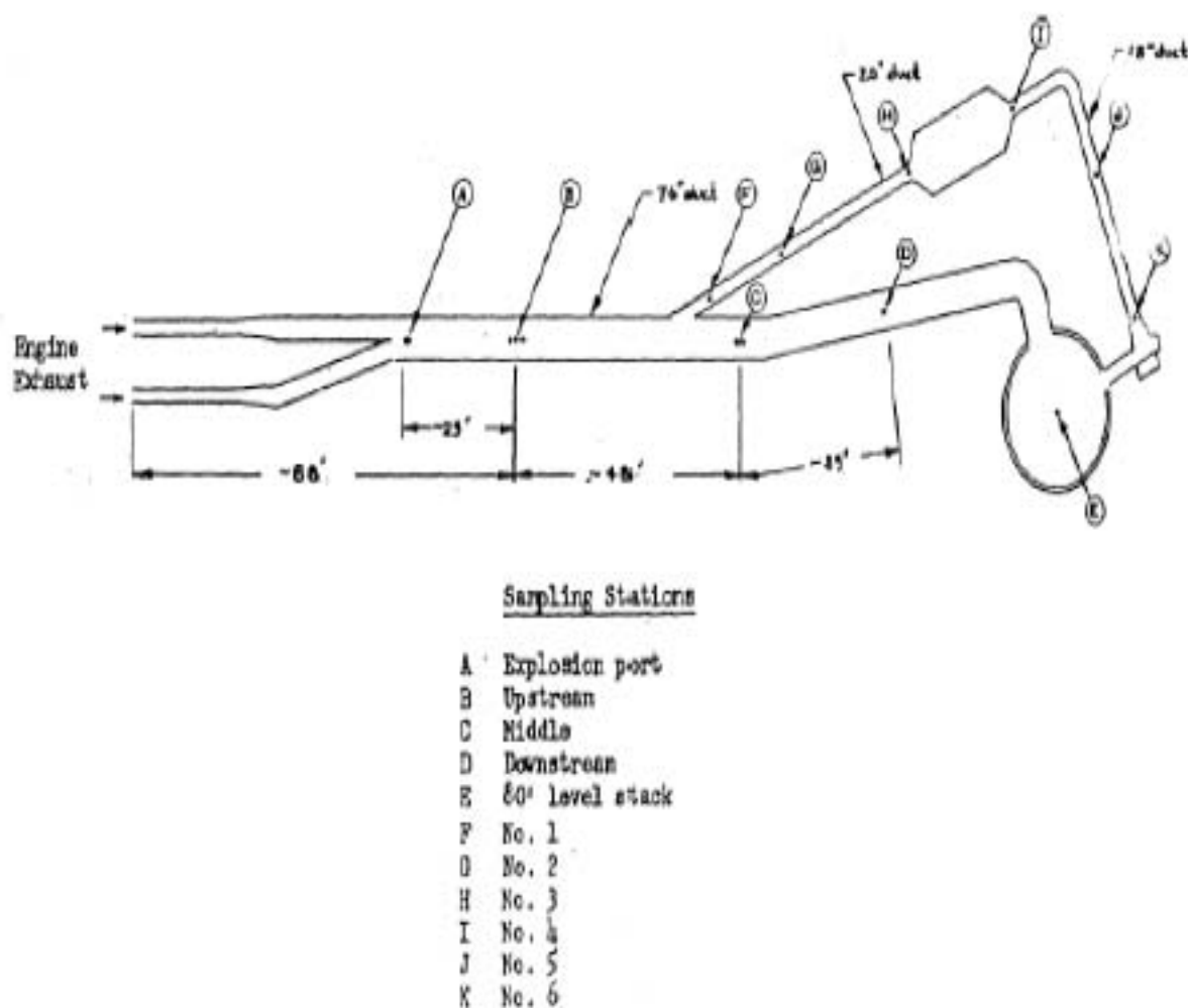
Figure 4-15 Nomenclature and Location of Limited Melt Experiment-II Sampling Station
