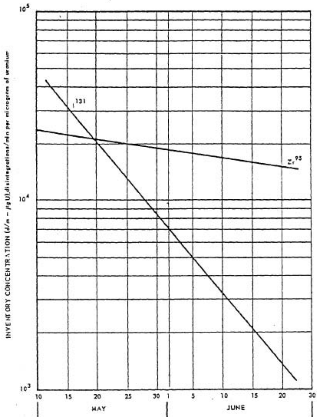
Figure B-27 Theoretical Inventory of I-131 and Zr-95 per Microgram of Uranium Remaining at Various Times After Melt
