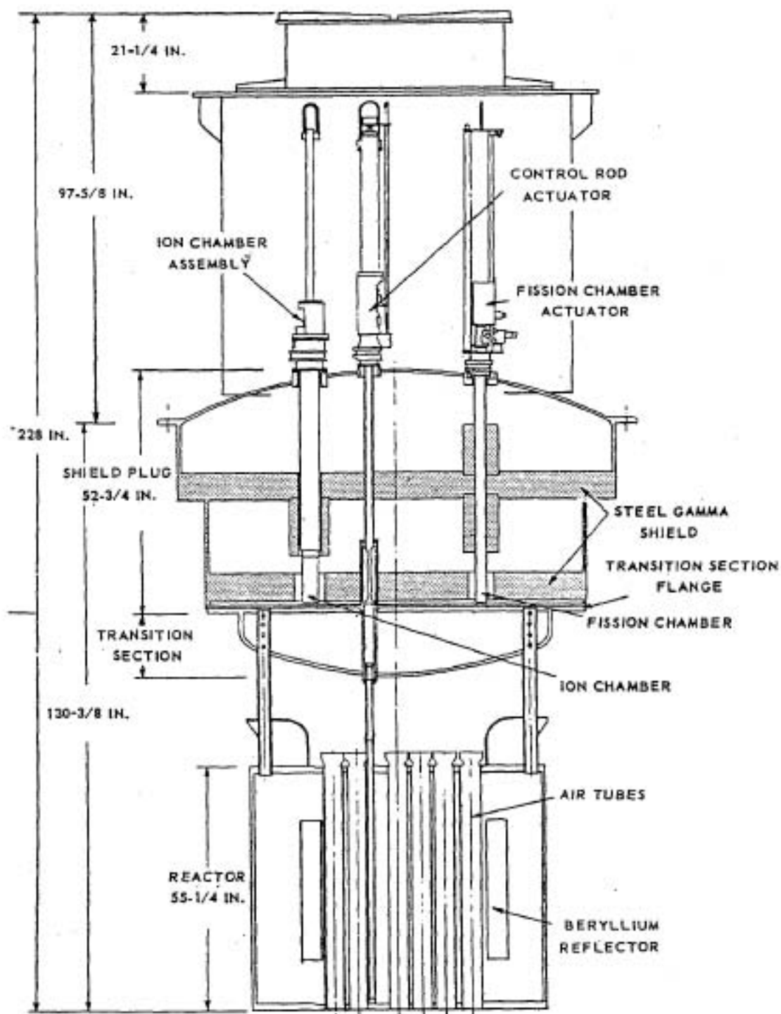
Figure 2-1 Schematic Drawing of Reactor Assembly
